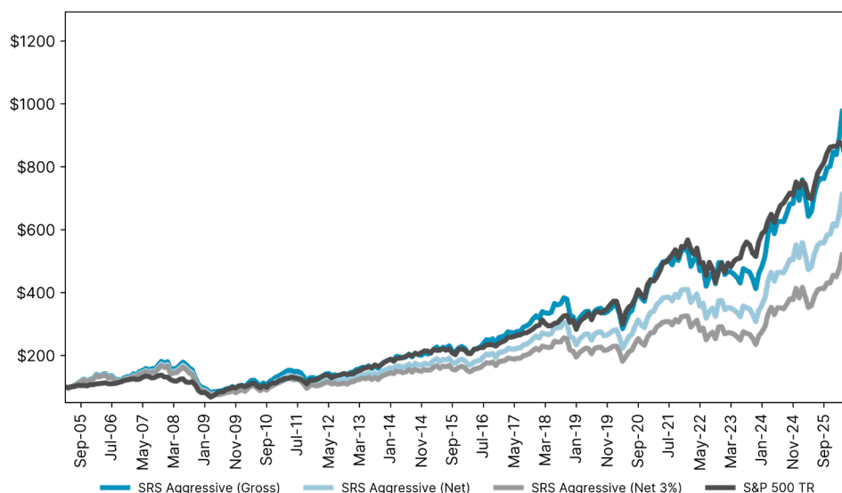
SRS Aggressive vs. S&P 500 (Mar 2005 - May 2026)
