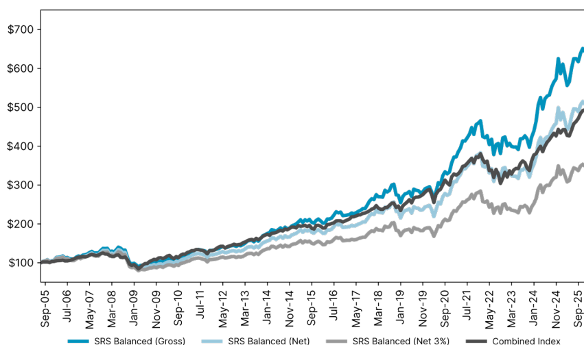
SRS Balanced vs. Combined Index (Jun 2005 - Jan 2026)
