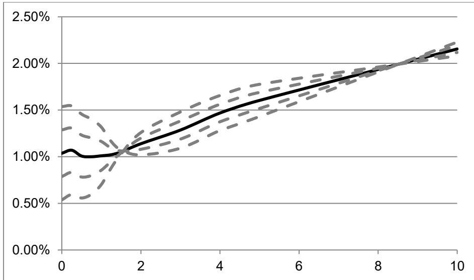
Figure 6. Stressing a curve with its third PC i.e. by different levels of curvature changes.
