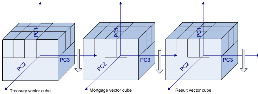
Figure 10. 3D window method applied on the treasury and mortgage vector cubes.
