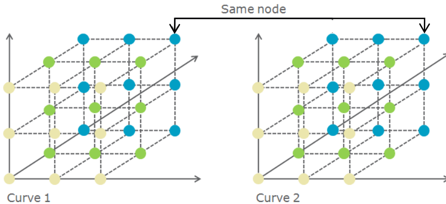
Figure 8. Example on two perfect correlated yield curves.
