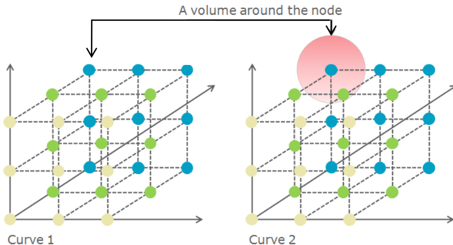
Figure 9. Example of two correlated curves.
